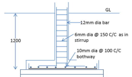
TYPICAL DETAILS OF RCC COLUMN
