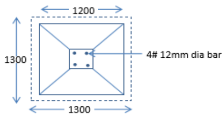
RCC COLUMN FOOTING
