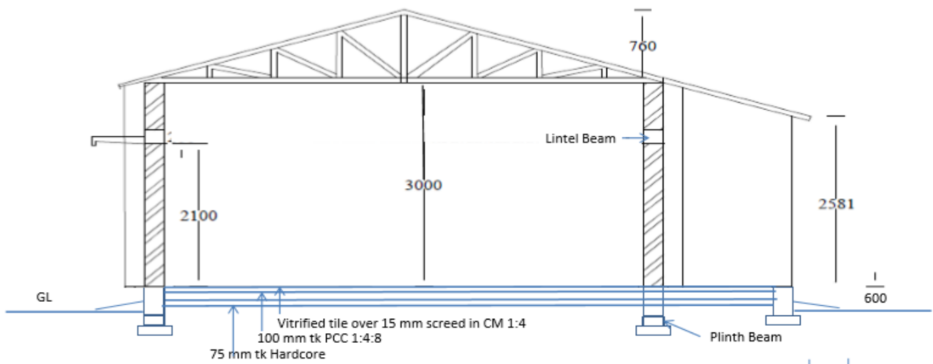
CROSS SECTION
